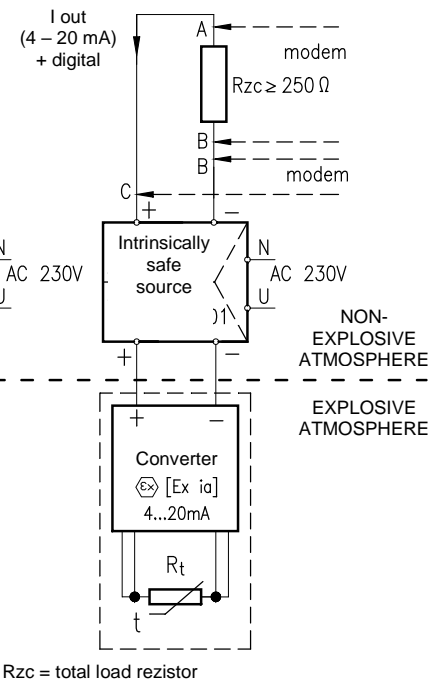
FIGURE 2- EXAMPLE OF OPERATION CONNECTION OF TEMPERATURE SENSOR WITH CONVERTER IN LOOP 4 - 20 mA
